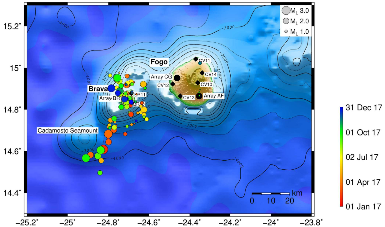
Figure 10. Earthquake locations from 18 January 2017 to 12 January 2018. Black circles: array locations; black diamonds: short-period single stations. Topography and bathymetry data are from Ryan et al. (2009).
