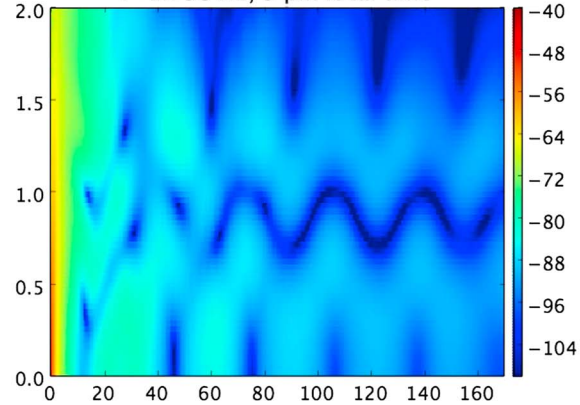
f) Range–elevation TL map f=1.758 Hz, 5 am local time
