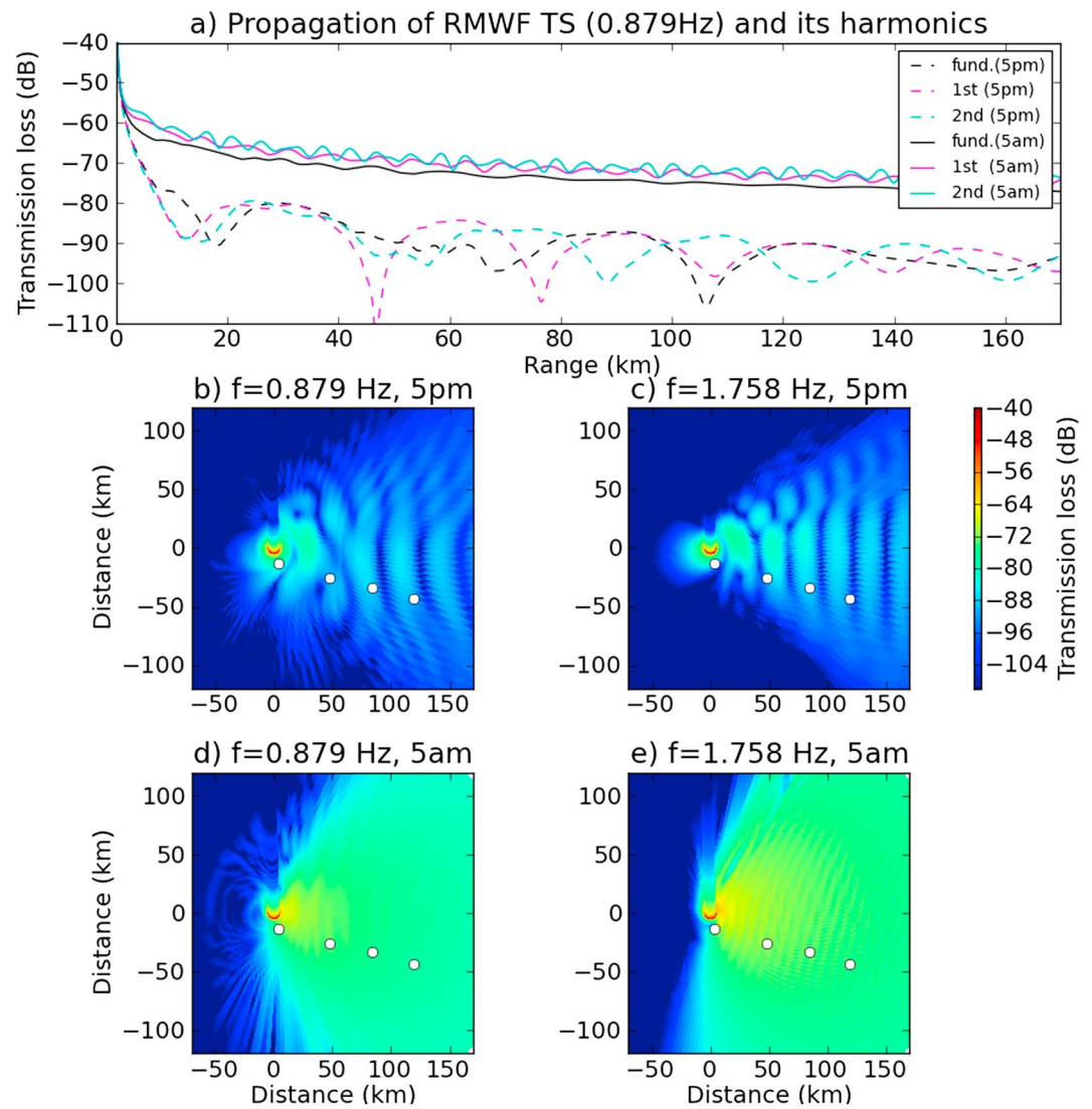
Figure 7. (a) TL profile at the ground for an azimuth of 113°, for the fundamental frequency (black), first (magenta), and second (cyan) harmonics; the radiosonde measurements correspond to those described in Figures 6a and 6d. TL (color-coded) at the ground for different ranges and azimuths for the fundamental frequency and first harmonic are shown for the (b and c) 05:00 P.M. and (d and e) 05:00 A.M. profiles. The location of the arrays (white dots) used in this experiment is shown relative to the wind farm.
