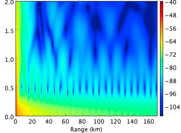
Figure 6. (a and d) Adiabatic and effective sound speeds (dashed and solid black lines) and zonal ( u ) and meridional ( v ) wind component (dashed and solid magenta lines) profiles for the Albuquerque radiosonde data corresponding to 17 and 18 February at 05:00 P.M. and 05:00 A.M., respectively (LST). (b, c, e, and f) Range–elevation transmission loss (TL) maps for the fundamental and first harmonic frequencies.
